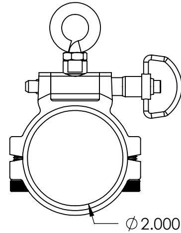
03-1154-23TQ 2" Teaser Clamp Tournament Outrigger Main Base Tube (Below 1st Spreader)
