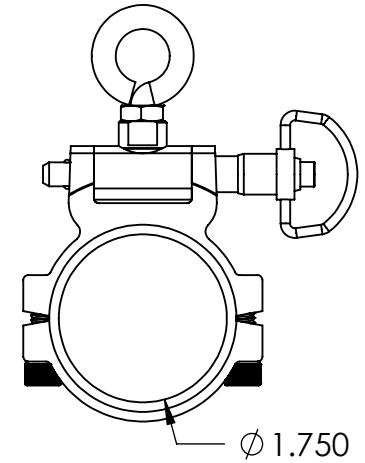
03-1856-23TQ 1 3/4" Teaser Clamp Tournament Outrigger Lower Intermediate Tube (Above 1st Spreader)
