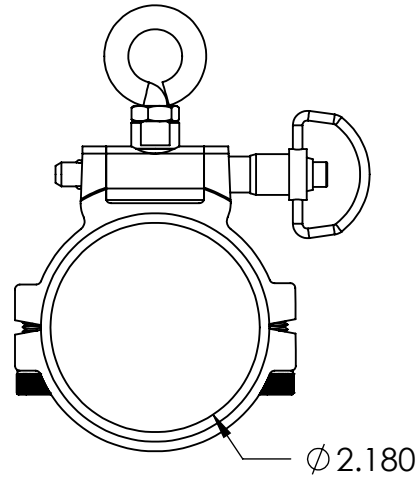
03-1528-23TQ 2 3/16" Teaser Clamp Bigg Rigg Outrigger Lower Intermediate Tube (Above 1st Spreader)
